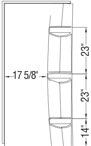
Wall A
